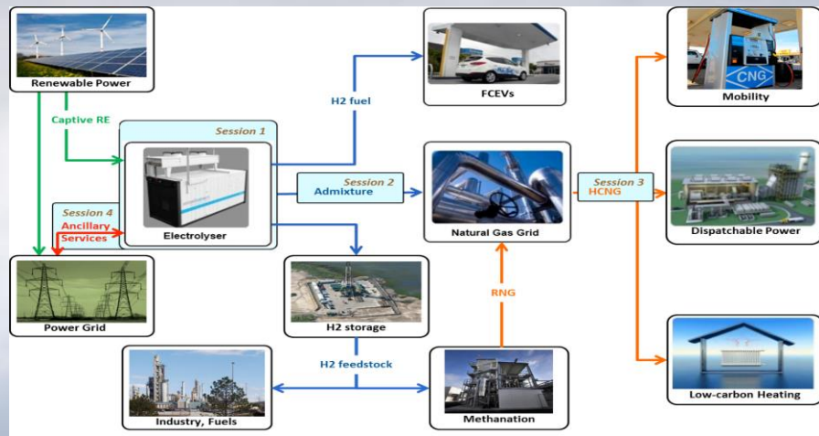
P2H Diagram developed by JRC, October 2014
